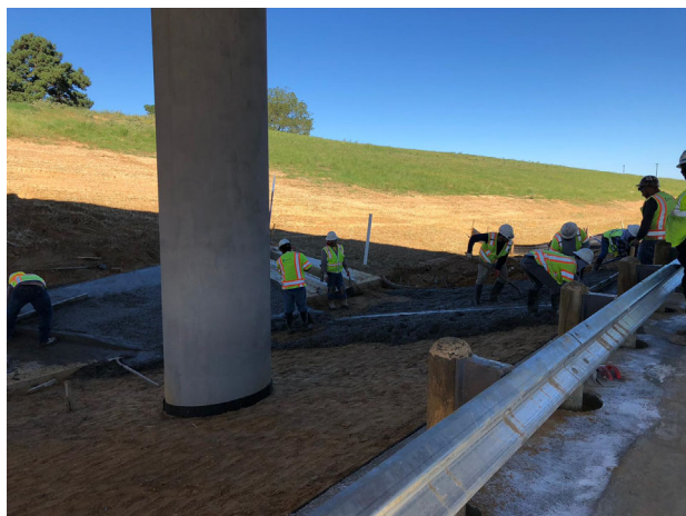
Concrete rip rap placement at FM 849 Abutment
