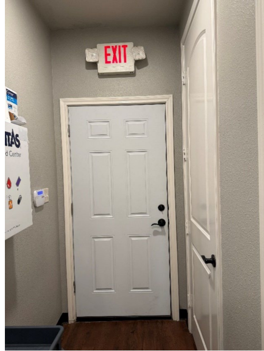
Corridor does not allow for required door clearance at emergency exit. 18" min. required on latch side by TAS (below right).
