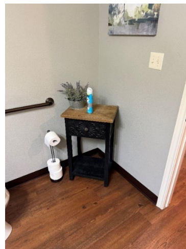
Required toilet clearance is obstructed by furniture fixture in back bathroom.
